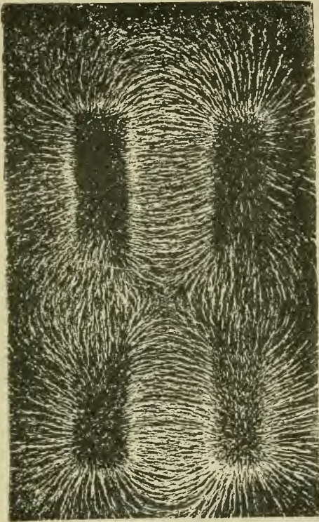
MAGNETIC FIELDS OF FORCE.
